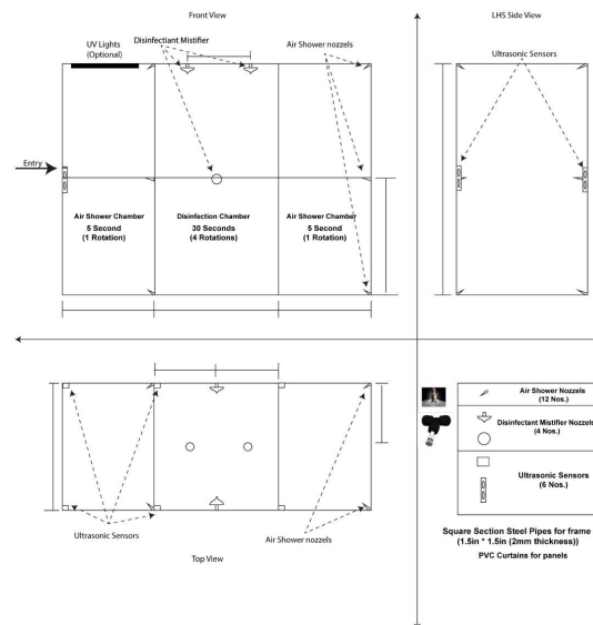
2-D Drawing of the Disinfection Chamber
